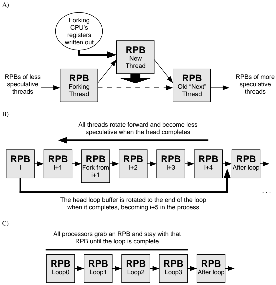
Figure C-3: Managing the register passing buffers (RPBs). A) During a subroutine fork. B) During a “slow” loop. C) During a “quick” loop.
