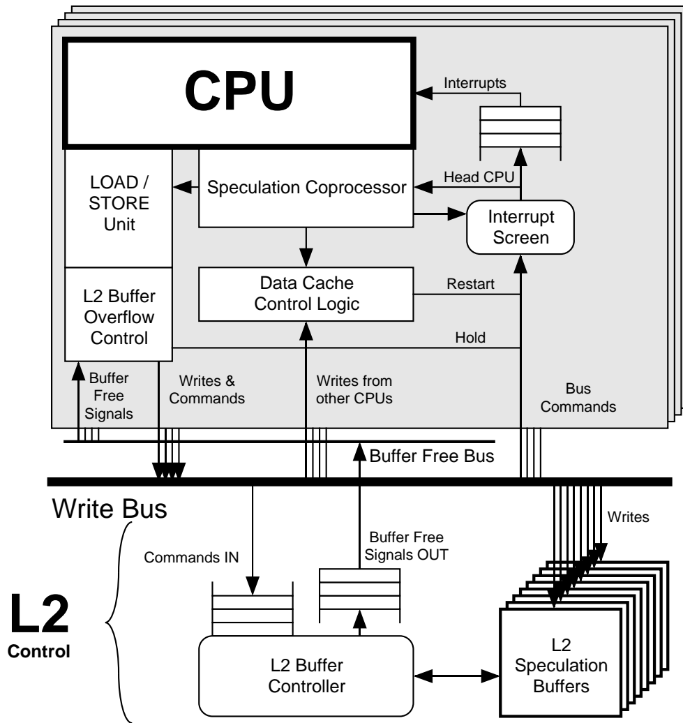
Figure 4-5: An overview of the speculation hardware added to Hydra
