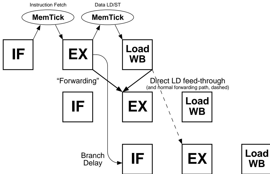
Figure A-2: The LESS Pipeline
