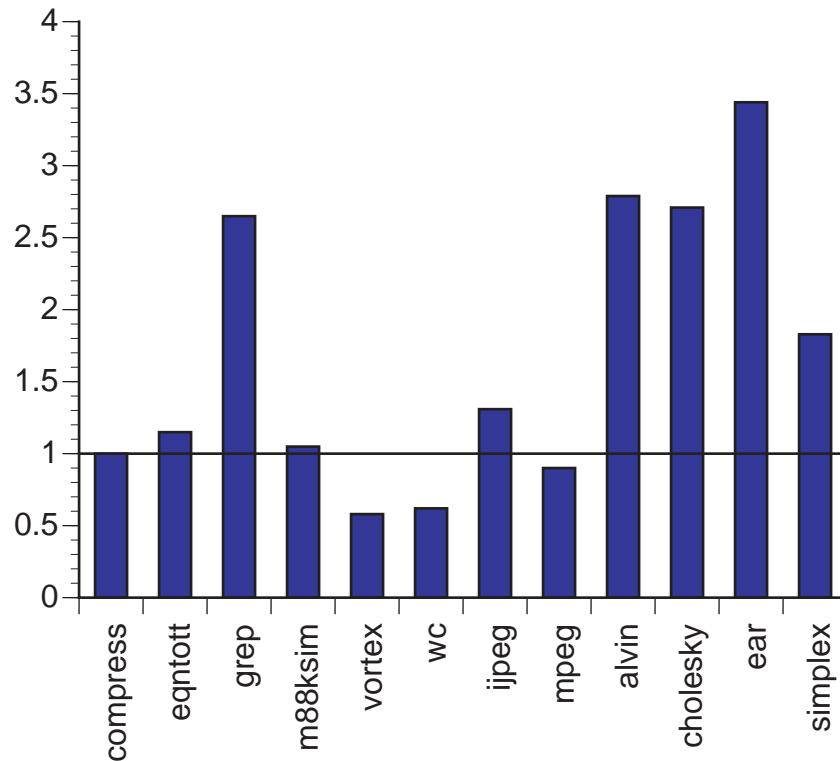
Figure 6-1: Baseline speculation system performance, in speedup of 4-processor system over a single processor executing the original uniprocessor benchmark.
