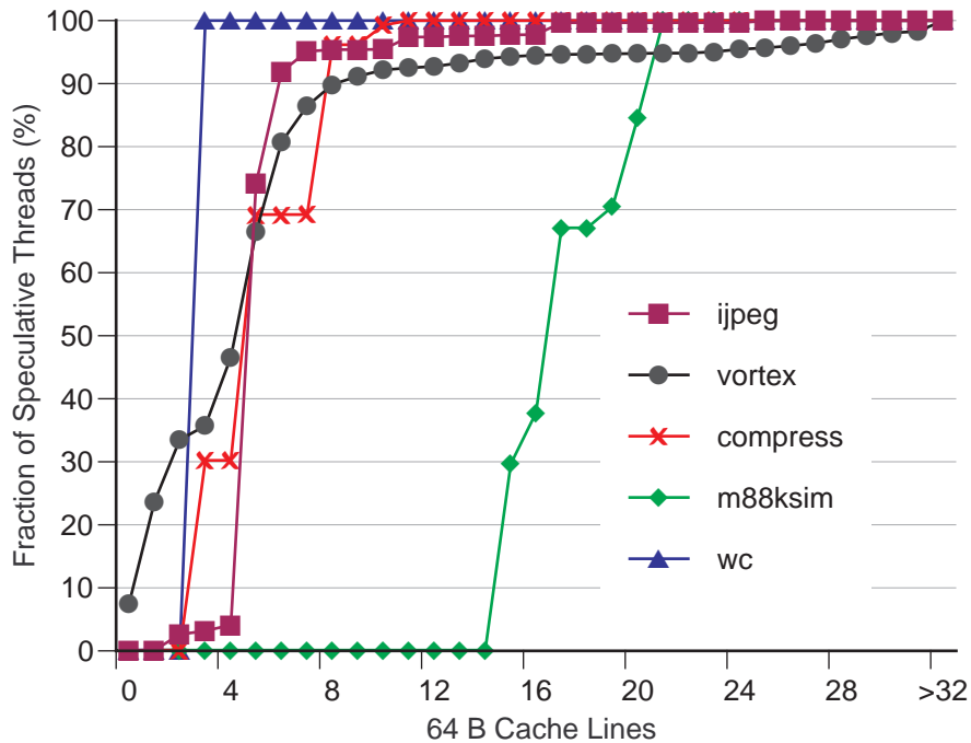
Figure 6-3: Speculative store buffer size requirements for some benchmarks.
