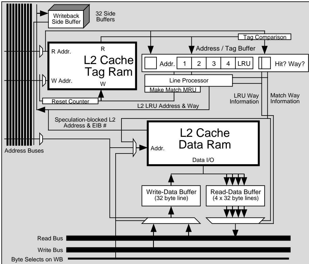
Figure B-9: The structure of the Hydra L2 cache
