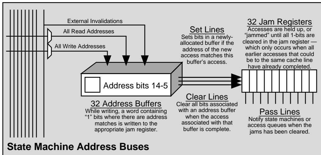
Figure B-6: The address-check buffers in the Hydra chip
