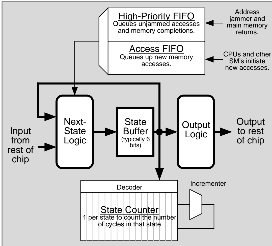
Figure B-7: A typical state machine that controls the memory system
