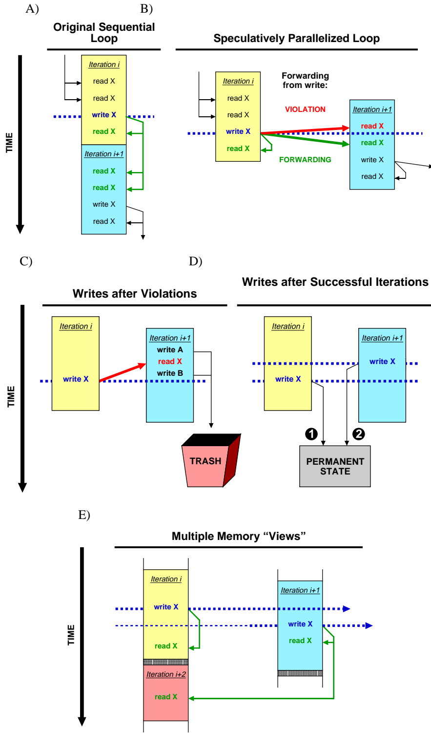
Figure 4-2: Diagrams illustrating the five critical requirements that must be handled in a speculatively parallel memory system using a sample thread that can be broken into two speculative threads (a): b) Forwarding and violation detection on each memory reference, c) discarding of speculative state following a violation, d) reordering of writes following thread commits, and e) memory renaming among the threads.
