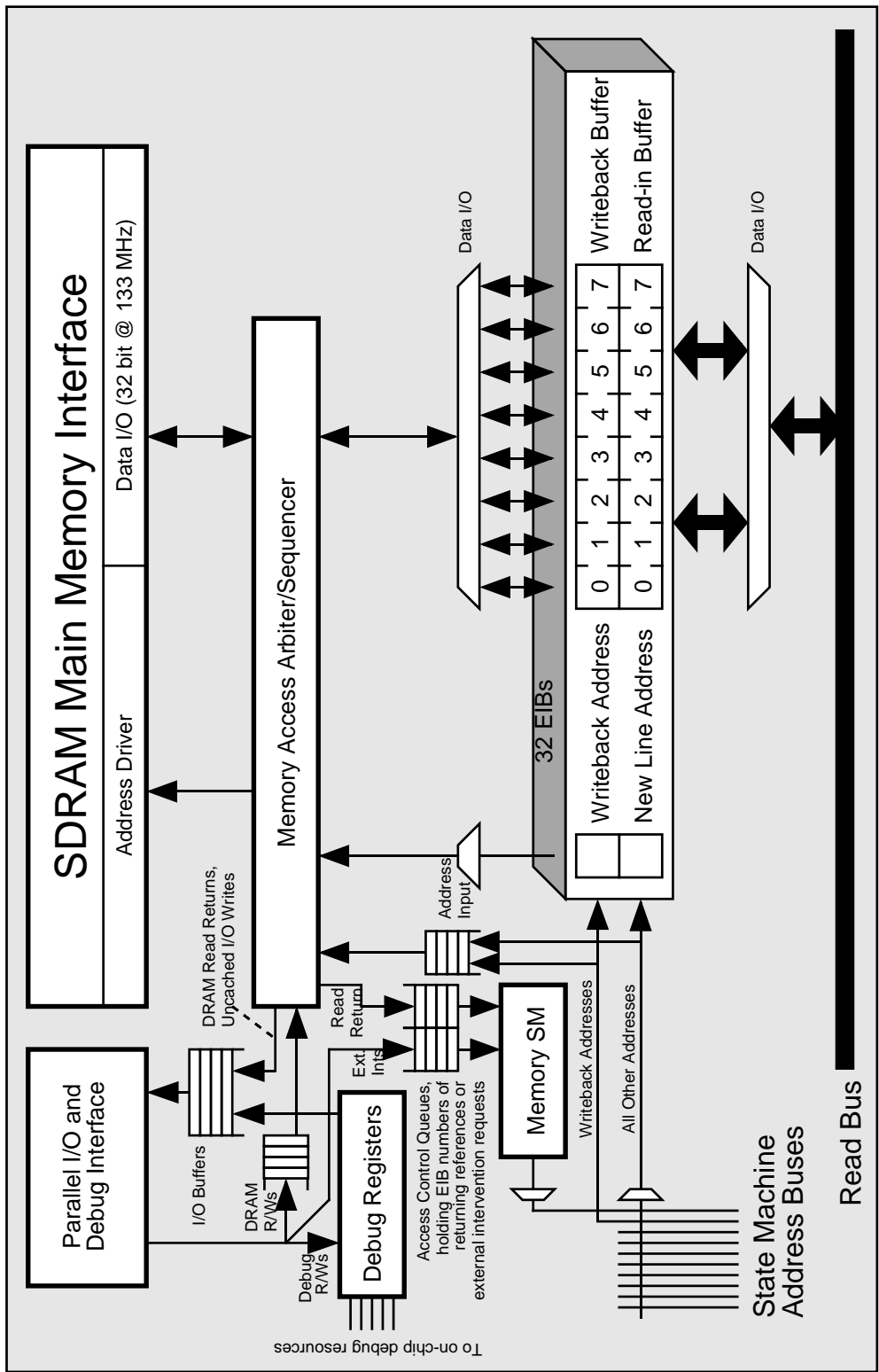
Figure B-10: Overview of the external memory and testing interface.
