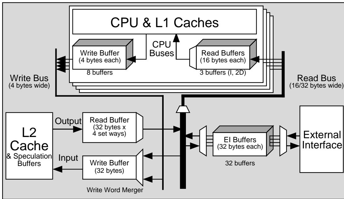
Figure B-3: A summary of the data buses that connect the parts of Hydra together.
