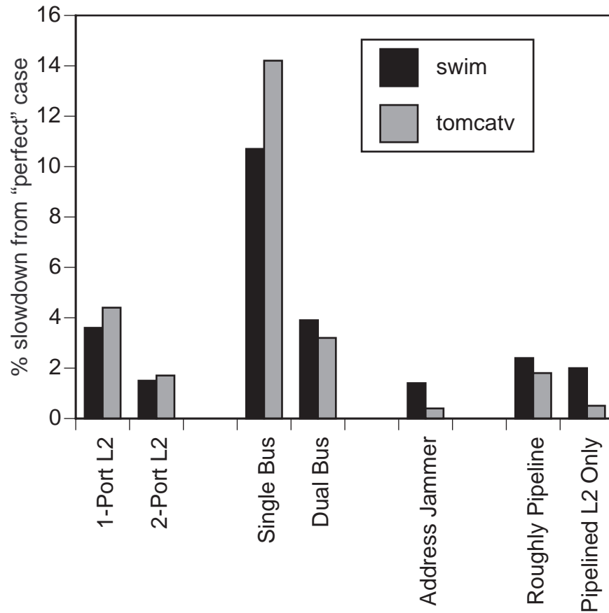
Figure 3-3: The % increase in execution time seen as a result of making several realistic architectural decisions, over “perfect” scenarios.
