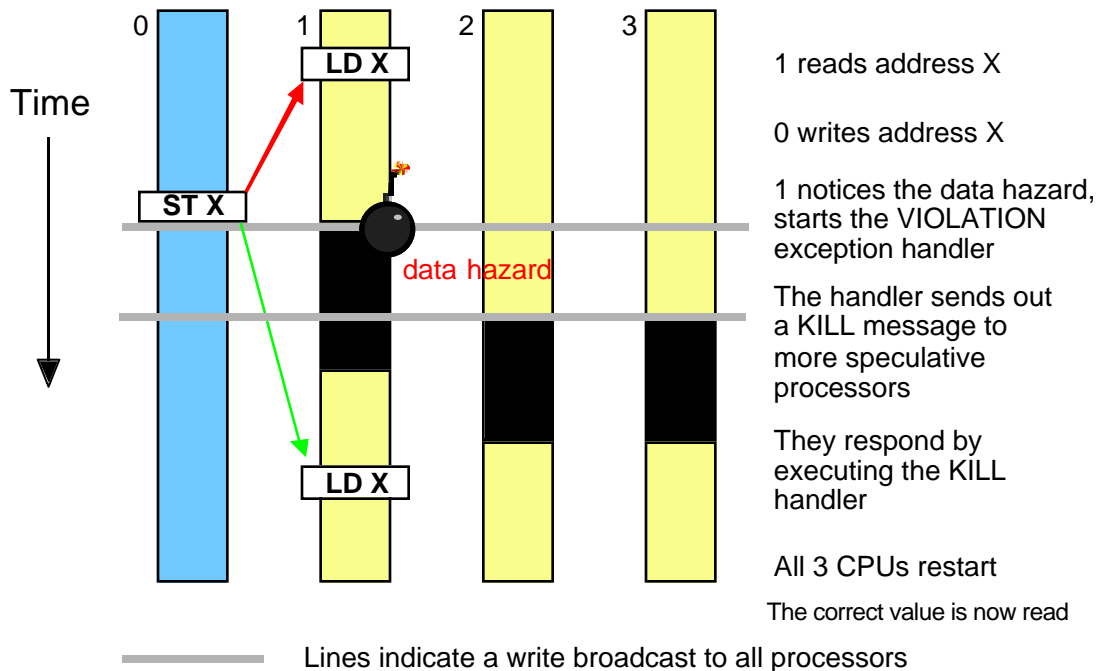
Figure 4-12: The sequence of events during a typical speculative violation
