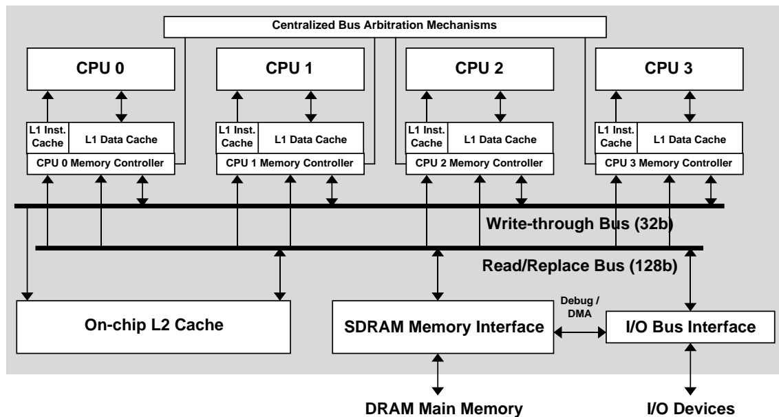
Figure 2-1: An overview diagram showing the major portions of Hydra and how they interconnect through the read and write buses.
