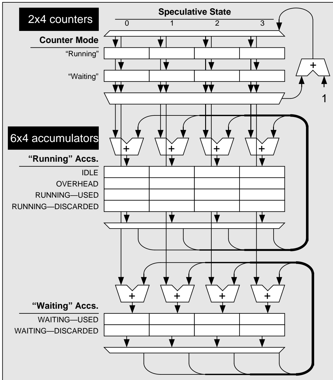
Figure C-1: A schematic overview of the state-time accumulator system
