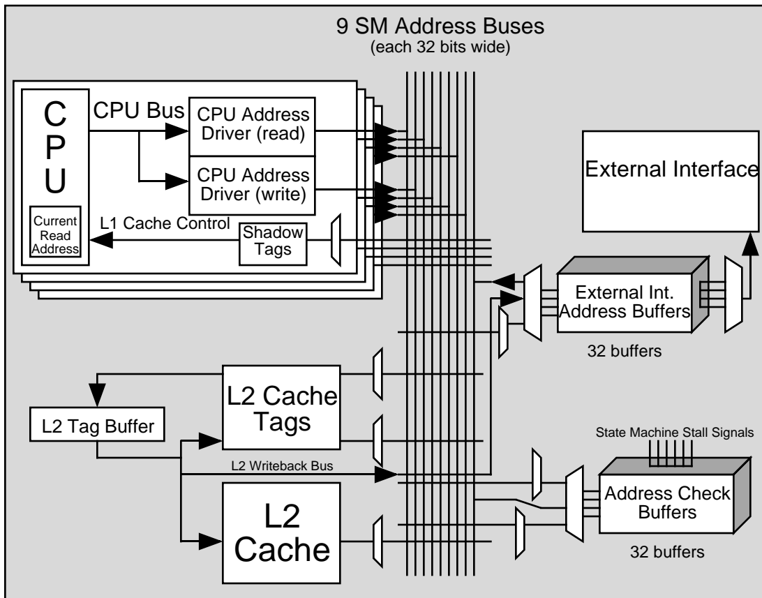
Figure B-4: A summary of the address resources in Hydra
