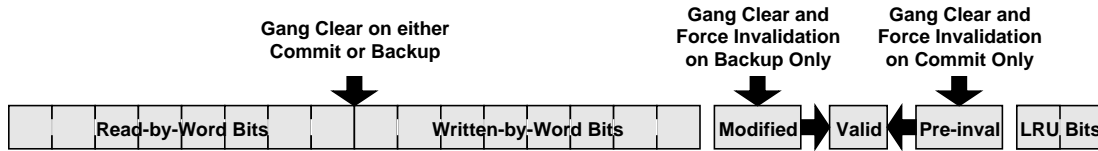
Figure 4-6: Speculation control bits supplementing the L1 cache tags.
