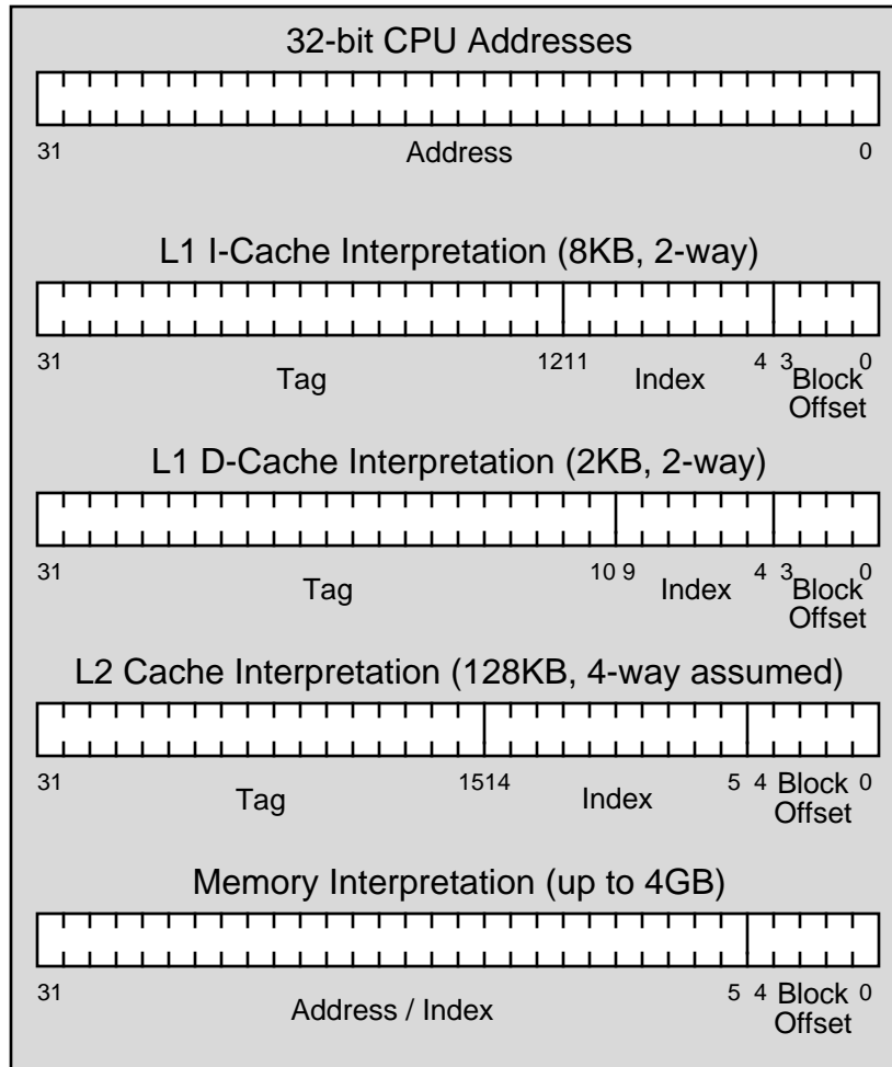
Figure B-5: Address formats at different levels of the Hydra cache hierarchy
