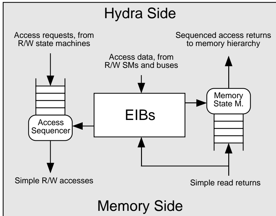
Figure B-8: Flow of memory references through the main memory interface.
