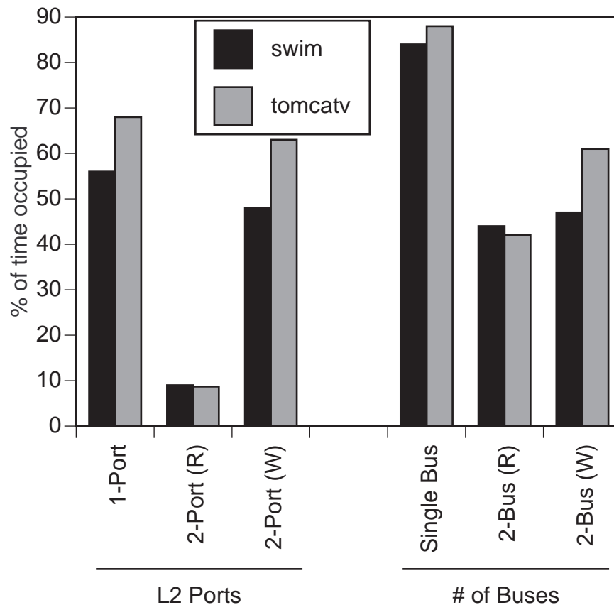
Figure 3-2: The occupancy of L2 cache ports and buses during runs.
