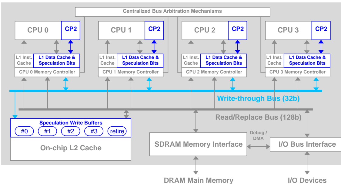
Figure 4-1: An overview diagram of Hydra, with additions required to support speculative threads highlighted.
