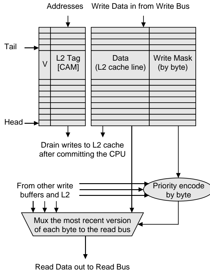
Figure 4-7: Block diagram of a single write buffer (1 of 8)
