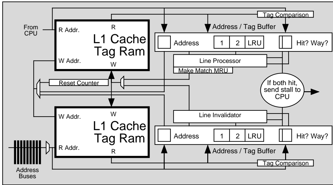
Figure B-1: The enhanced L1 data cache tag system.
