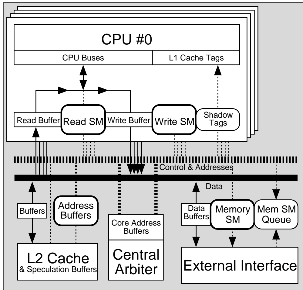
Figure B-2: An overview of the Hydra memory interconnection system.
